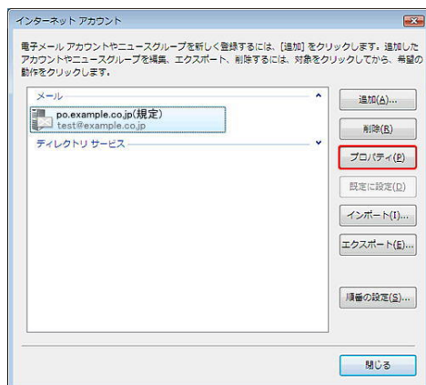
Windows mail
