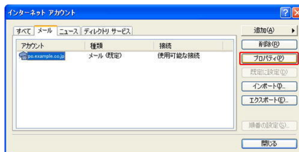
Outlook Express
